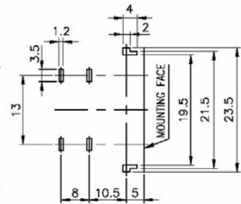
P.C. BOARD MOUNTING HOLD DIMENSION
